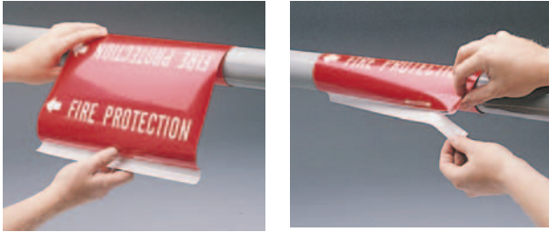
B-689 High Performance Pipe Markers are pre-coiled for easy wrap-around installation on pipe up to 7 7/8" in diameter.
