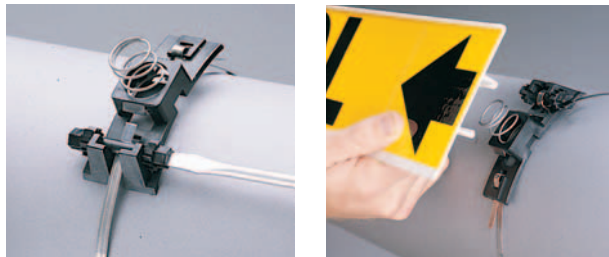
High Performance B-681 labels with overlaminated graphics are factory applied to a fiberglass plastic carrier for easy strap-on installation on pipes 8" and larger in diameter.
